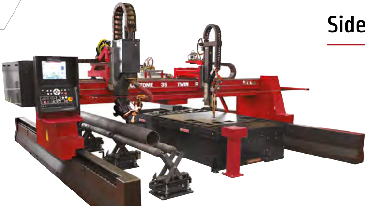
Plasma cutting system with tube cutting
