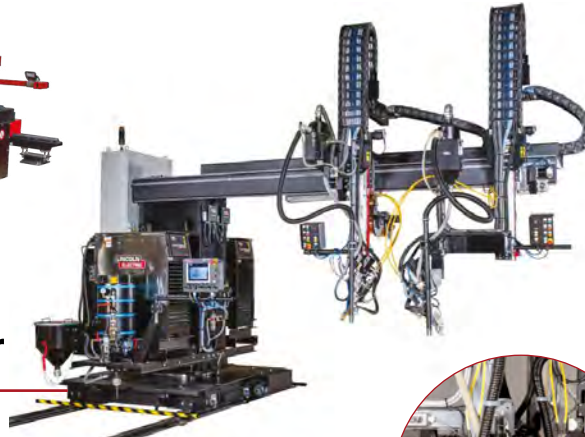
Beam welder
